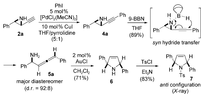
Scheme 1. Preparation of an internal \alpha -amino allene for elucidation of the relative stereochemistry.
