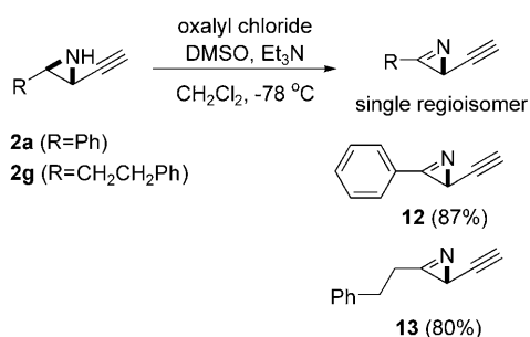
Scheme 3. Chemoselective and regioselective azirine synthesis from N–H ethynylaziridines.
