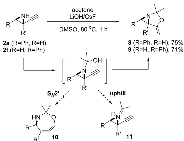
Scheme 2. Annulation of N–H ethynylaziridines with acetone.
